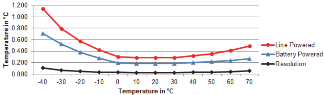
Plot A: Accuracy Range of ZW-001 Integrated Temperature Sensor
