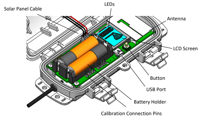
Sensor Mote Opened
